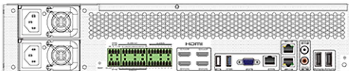
Rear panel for redundant series
